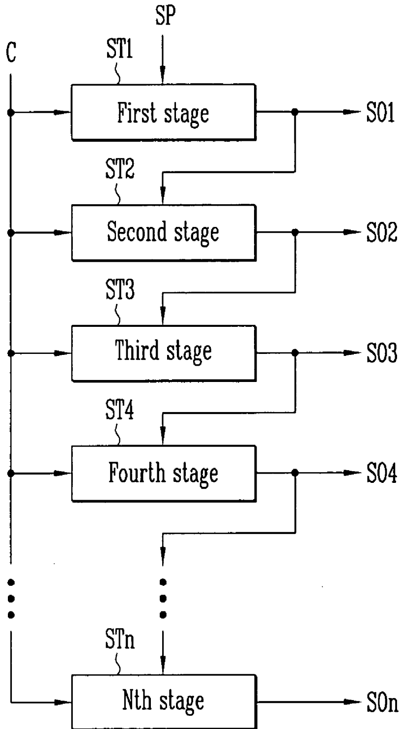
FIG. 1 (PRIOR ART)
